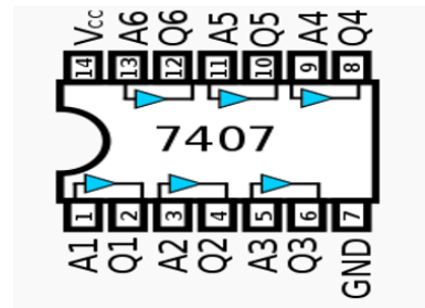
BUFFER
