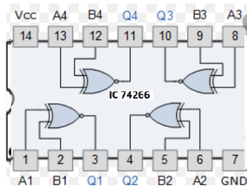
XNOR
